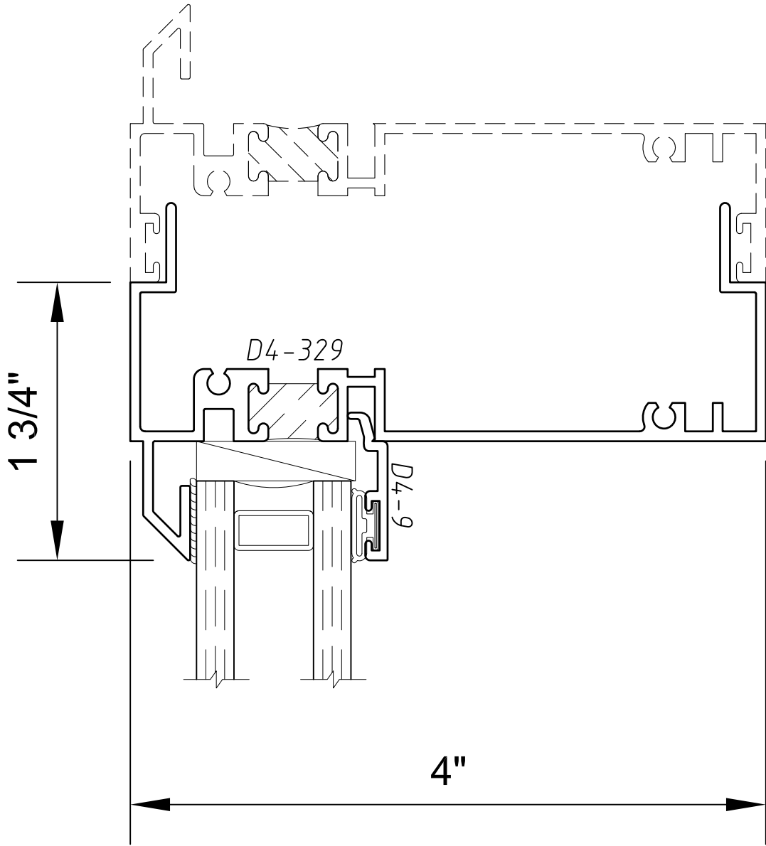
Horizontal stack section
